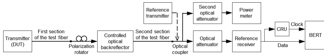
Figure B.3. Test setup for measurement of transmitter and dispersion penalty in the nonlinear power regime of the fiber.
