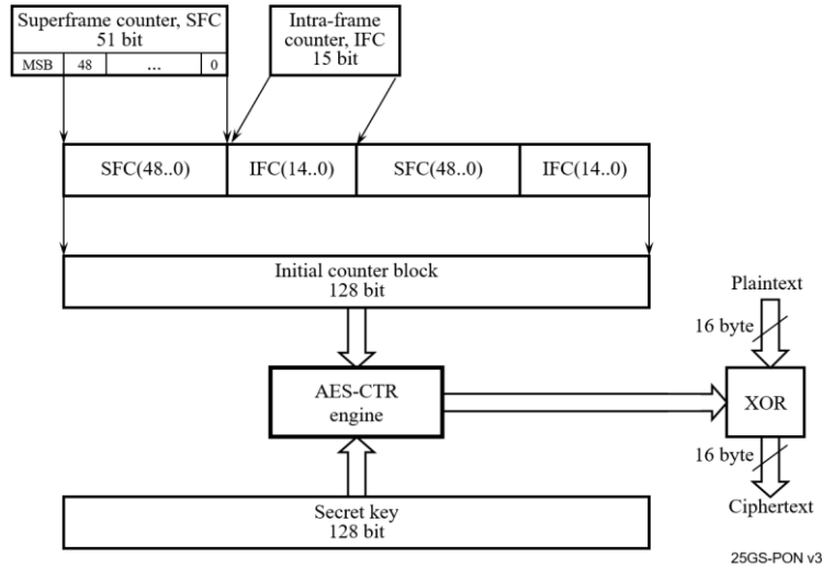
Figure C.15.2a – Initial counter block construction for downstream encryption
